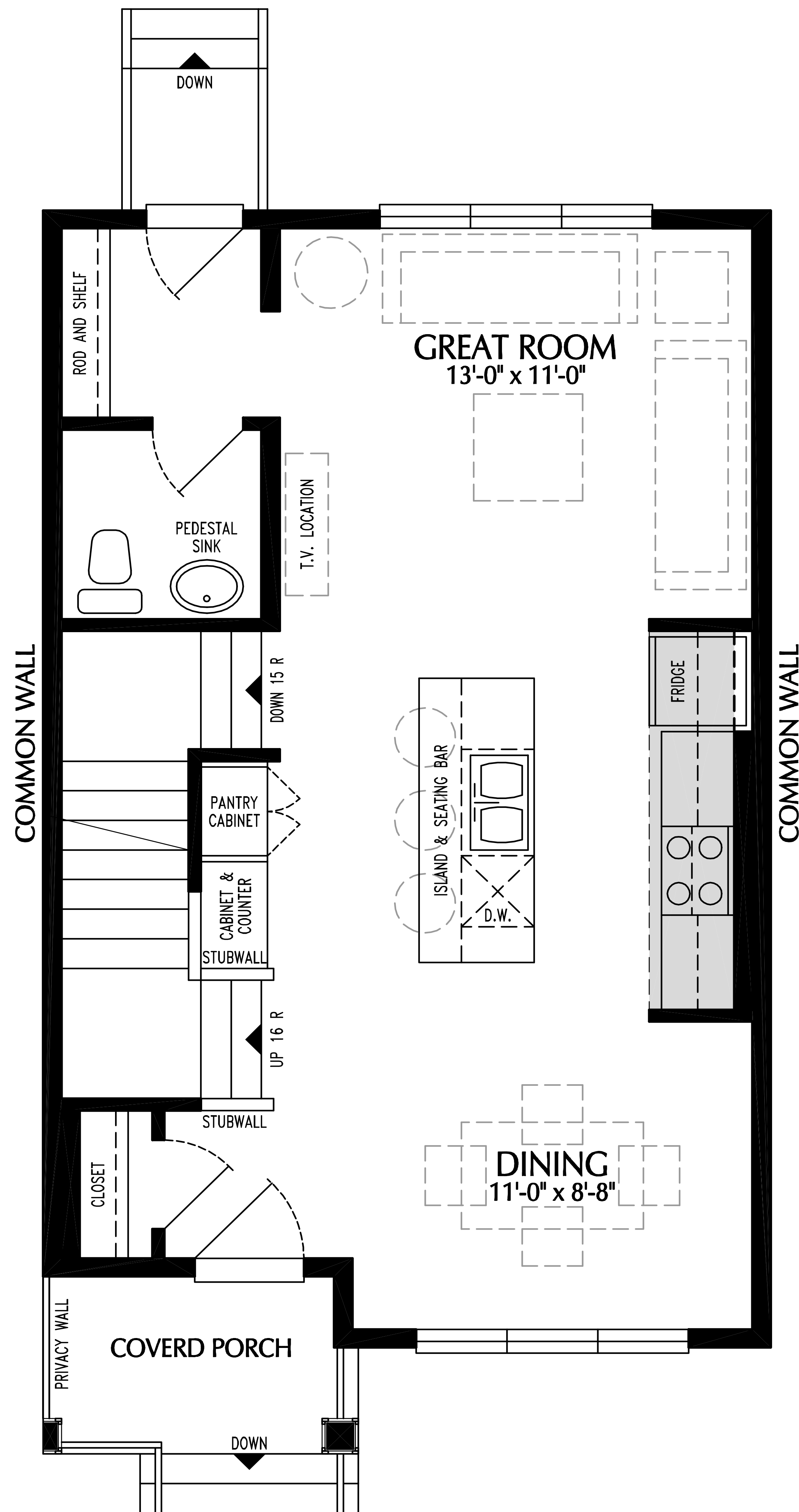
MAIN FLOOR PLAN 624 sq.ft.
